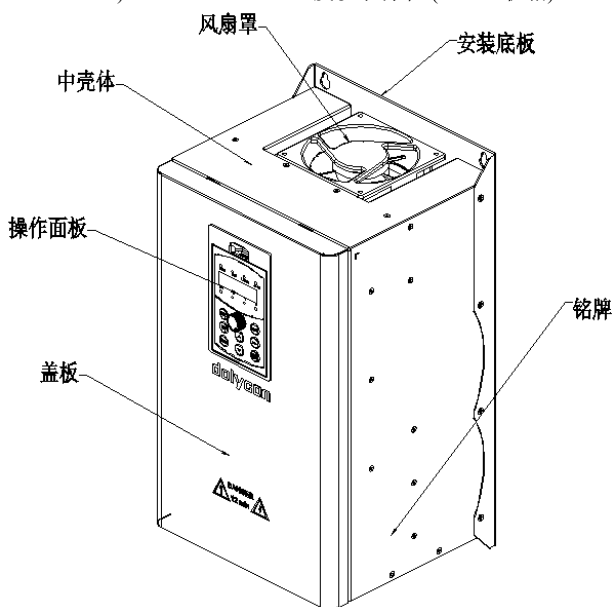
b) CT200-4T-15G-B ~ CT200-4T-37G-B (C3/C4 机箱)
