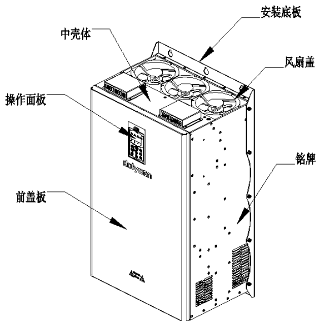
d) CT200-4T-132G~CT200-4T-200G (C7 机箱)
