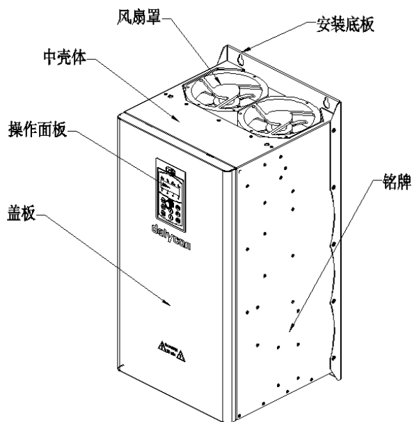
c) CT200-4T-45G~CT200-4T-110G (C5/C6/C7 机箱)
