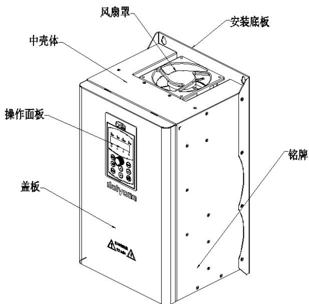
b) CT110-4T-15G/18.5P-B ~ CT110-4T-37G/45P-B (C3/C4 机箱)
