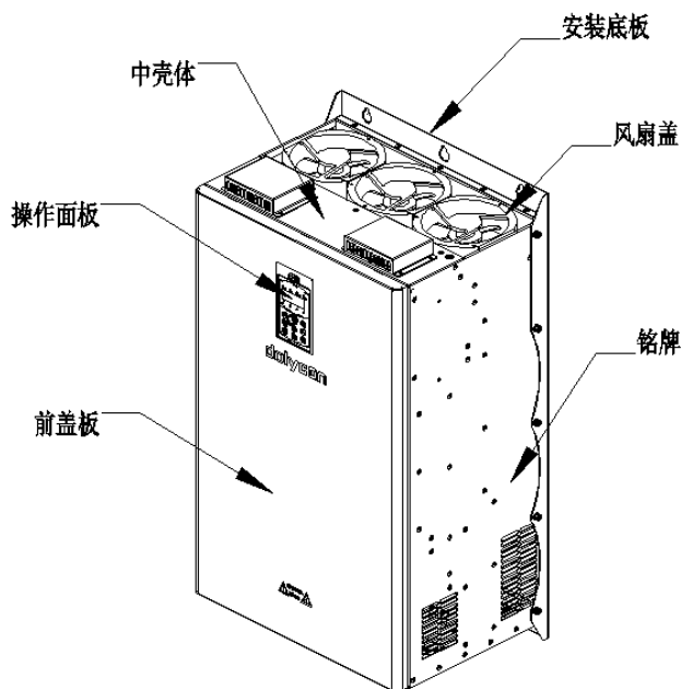
d) CT110-4T-132G/160P~CT110-4T-200G/220P (C7 机箱)
